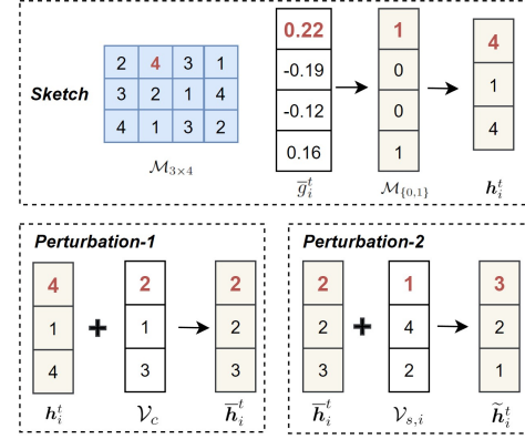
Fig. 6: A toy example of perturbed sketching with \epsilon = 0.1 .
