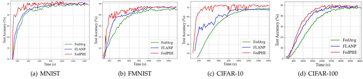
Fig. 10: Accuracy versus clock time of FedPHE and the baselines on different datasets.
